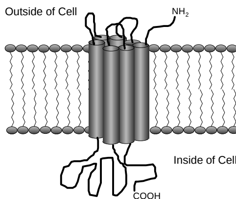
Figure 1. A schematic representation of a membrane-bound G-protein coupled receptor, of which the serotonin 5-HT 2A receptor is an example. The receptor consists of 7 alpha helices, represented here by tubes, connected on the inside and outside with continuing loops of protein.
