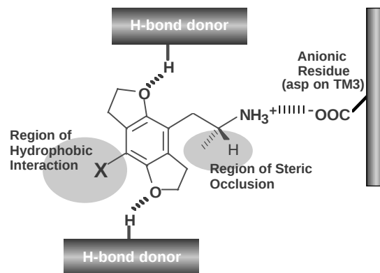
Figure 2. A schematic representation of a phenethylamine hallucinogen similar to DOB interacting with the ligand binding domain of the serotonin 5-HT 2A receptor. Important sites for chemical interaction include the amino group, the two oxygen atoms, the hydrophobic “X” group, and the central phenyl ring itself. Taken from Monte et al. 1996
