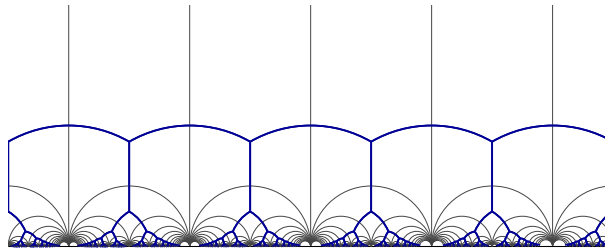
Figure A.3.2. The Voronoï decomposition and the retract in D
