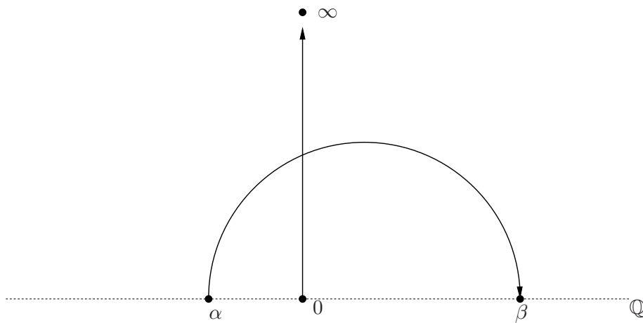
Figure 3.1.2. The modular symbols \{\alpha, \beta\} and \{0, \infty\} .
