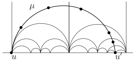
Figure A.6.2. A subdivision of \mu ; the solid dots are the x_i . Since the x_i lie in the same or adjacent Voronoï cells, we can assign cusps q_i to them to construct a homology to a cycle in \mathbf{C}_*^V .
