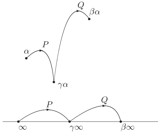
Figure 10.4.1. “Transporting” a transportable modular symbol.
