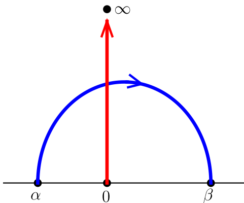
Figure 3.1.2. The modular symbols \{\alpha, \beta\} and \{0, \infty\} .
